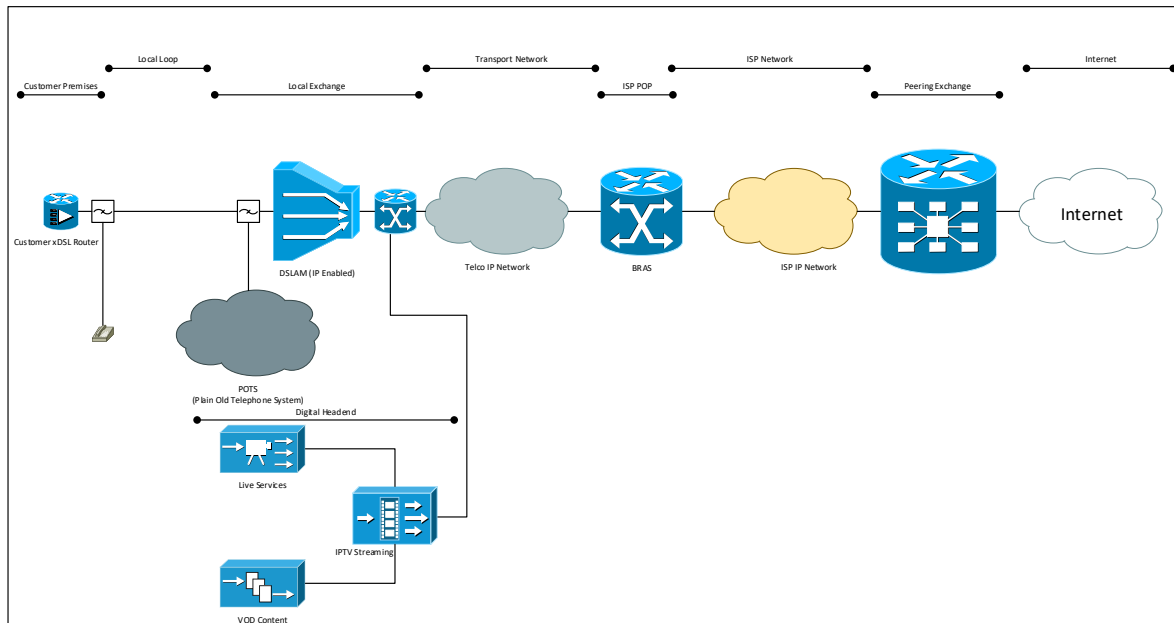
ISP Local Digital Headend IPTV Services at the Edge
