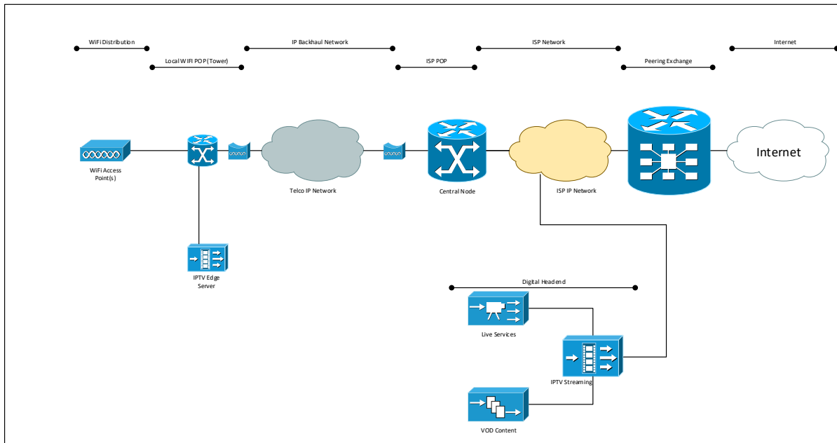
ISP Local Digital Headend IPTV Services
